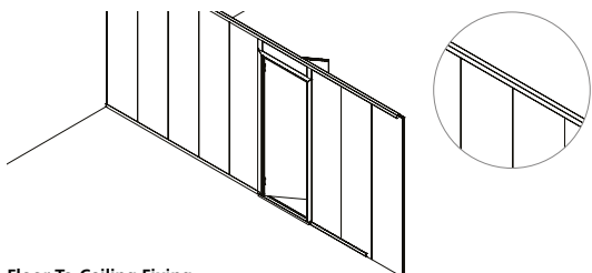
Floor-To-Ceiling Fixing U-Channel Top and Bottom
