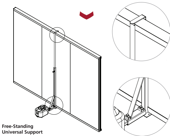
Floor-To-Ceiling Fixing U-Channel Top & Bottom
